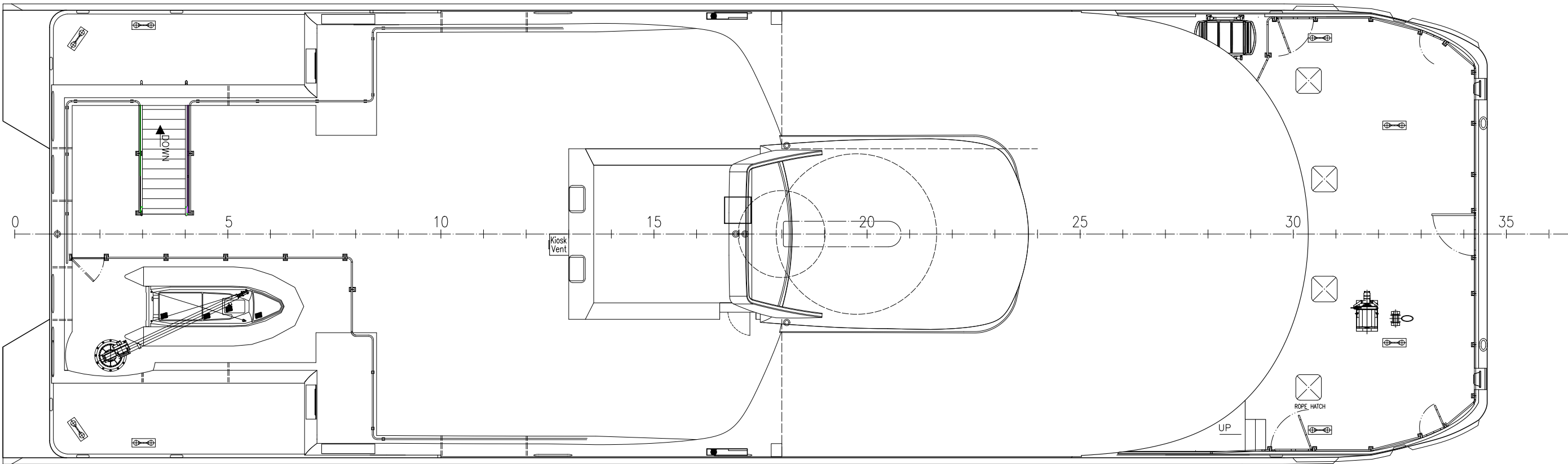
Topp dekk arrangement
