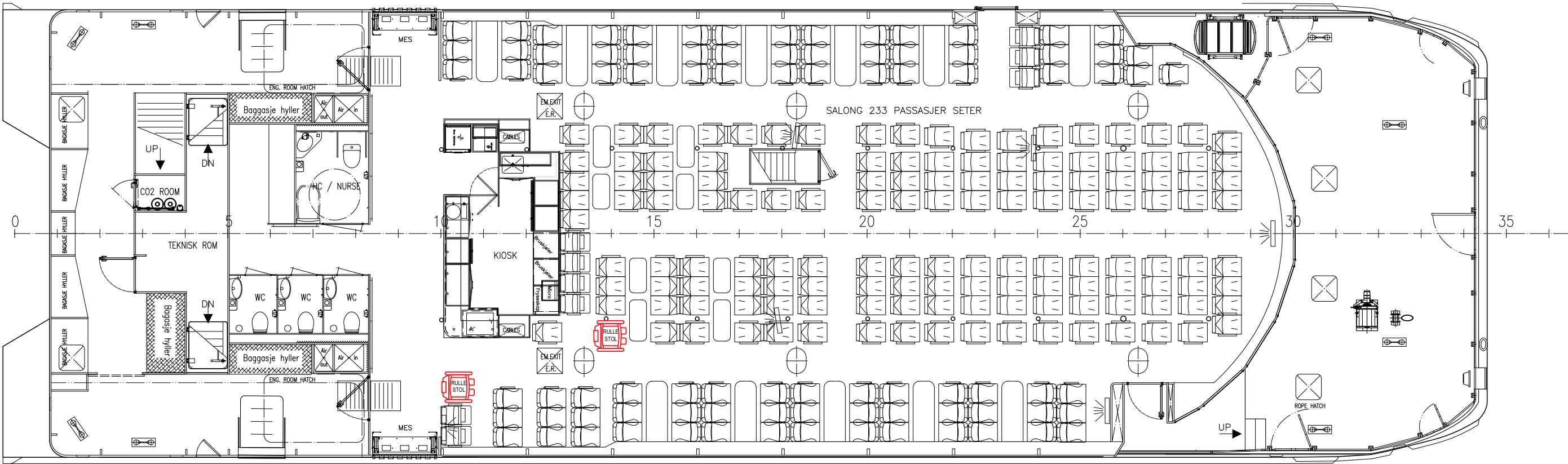
Hoved dekk arrangement
