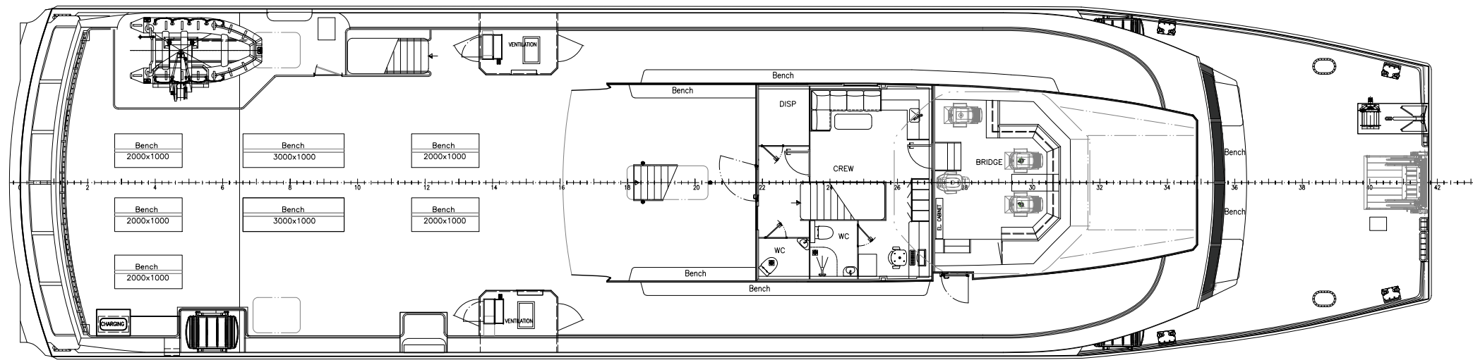
PLAN 01-DECK
