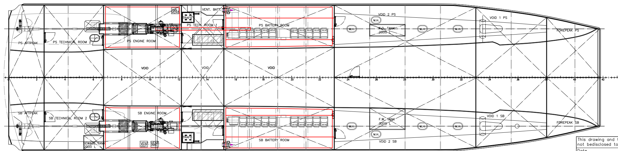
PLAN BELOW MAINDECK
