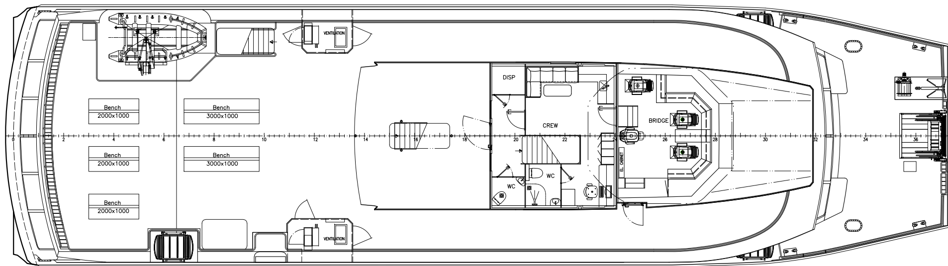
PLAN 01-DECK
