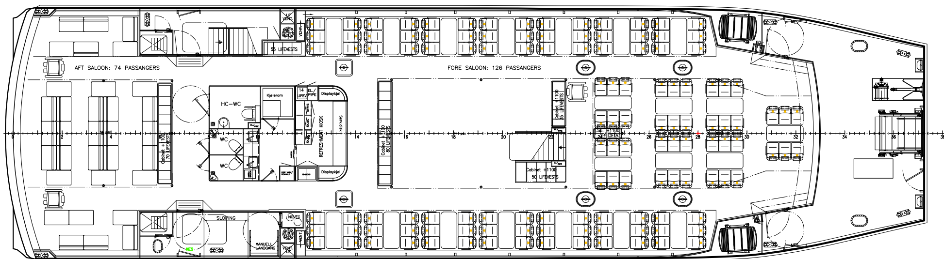
PLAN MAIN DECK (WINTER SIGHTSEEING AND RESTAURANT BUSINESS)
