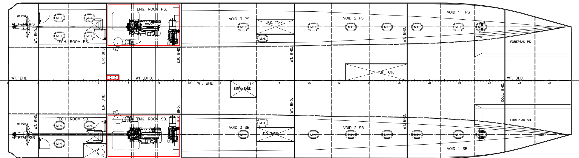
PLAN BELOW MAINDECK
