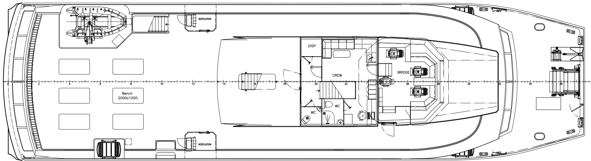
PLAN 01-DECK
