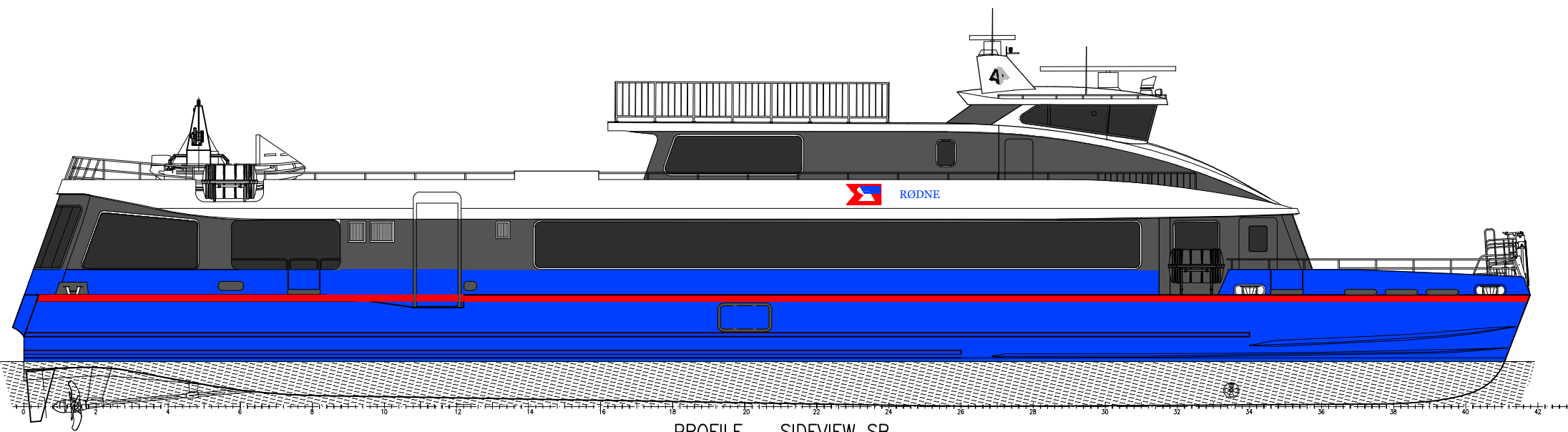
PROFILE – SIDEVIEW SB
